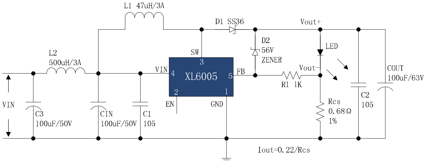
XL6005 VIN=DC5V~DC32V, IOUT=320mA Typical Application Circuit
